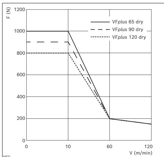
Permissible chain tensile force as a function of speed F(v) (N); max. 1000 N
